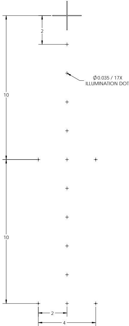
ILLULMINATION DETAIL
